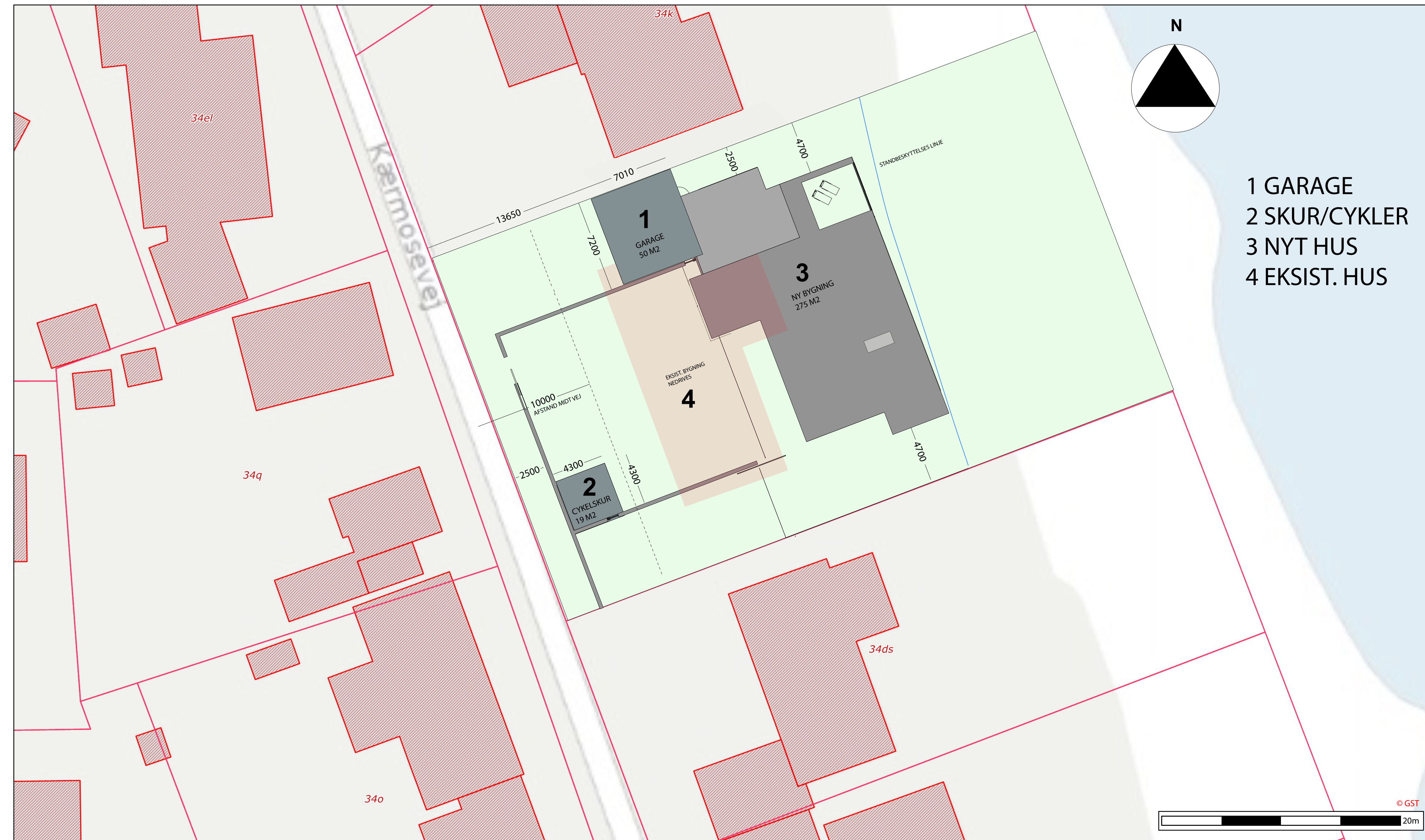
SITUATIONSPLAN 1:200
